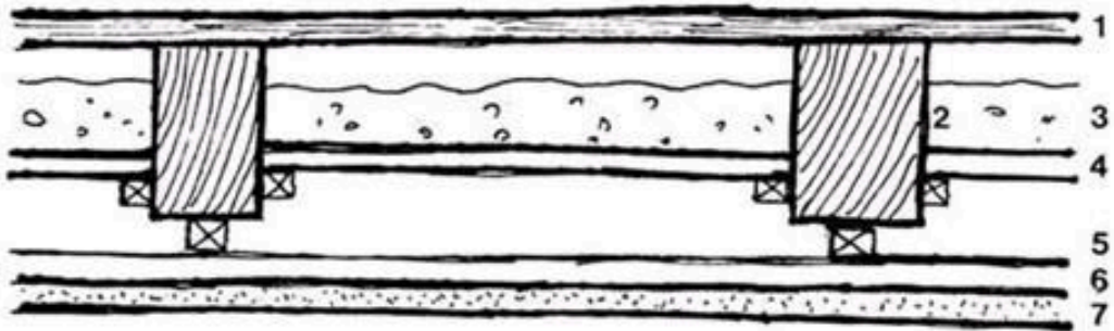
Sections of a traditional floor and a traditional roof in continental Greece and the islands of the Northern Aegean. In both cases earth in the structure's interior works as insulation. Floor: 1. Upper surface 2. Beams 3. Earth 4. Boards supporting the earth 5. Little beams 6-7 different layers of lime mortar
